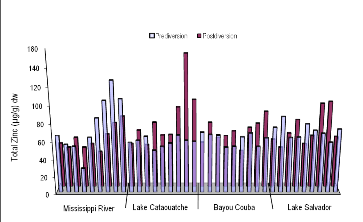
Figure 27B. Three-dimensional comparison of Davis Pond prediversion and postdiversion values for zinc by dry weight (in micrograms per gram [ \mu\text{g/g} ]).
